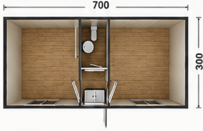
İZ306 MODEL
